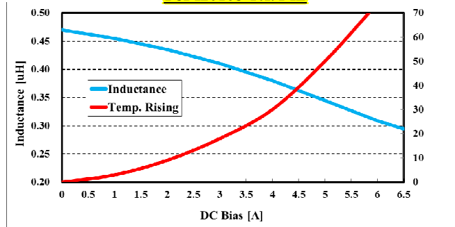
PSM2016S-R47ML
