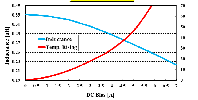
PSM2016S-R33ML
